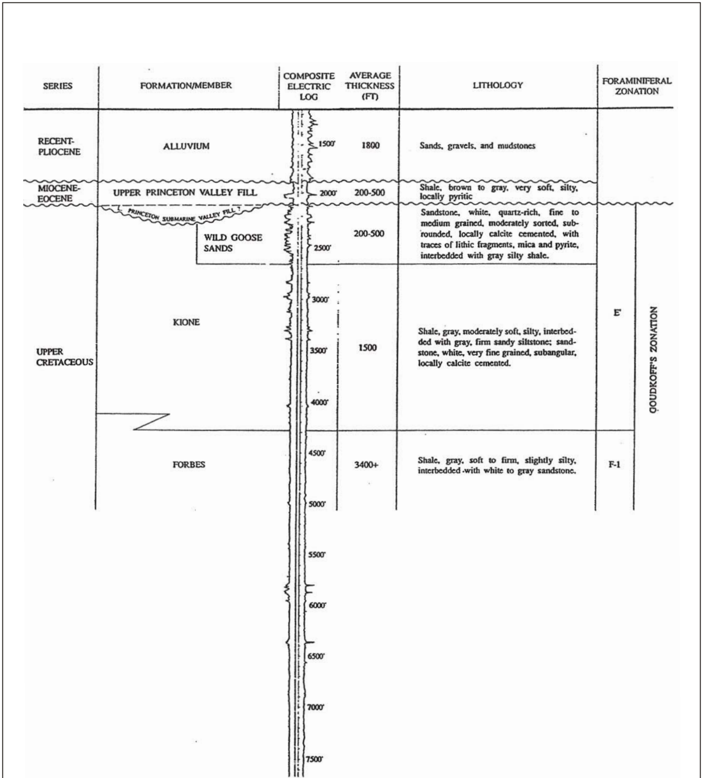
Stratigraphic column, Princeton Gas Field.
