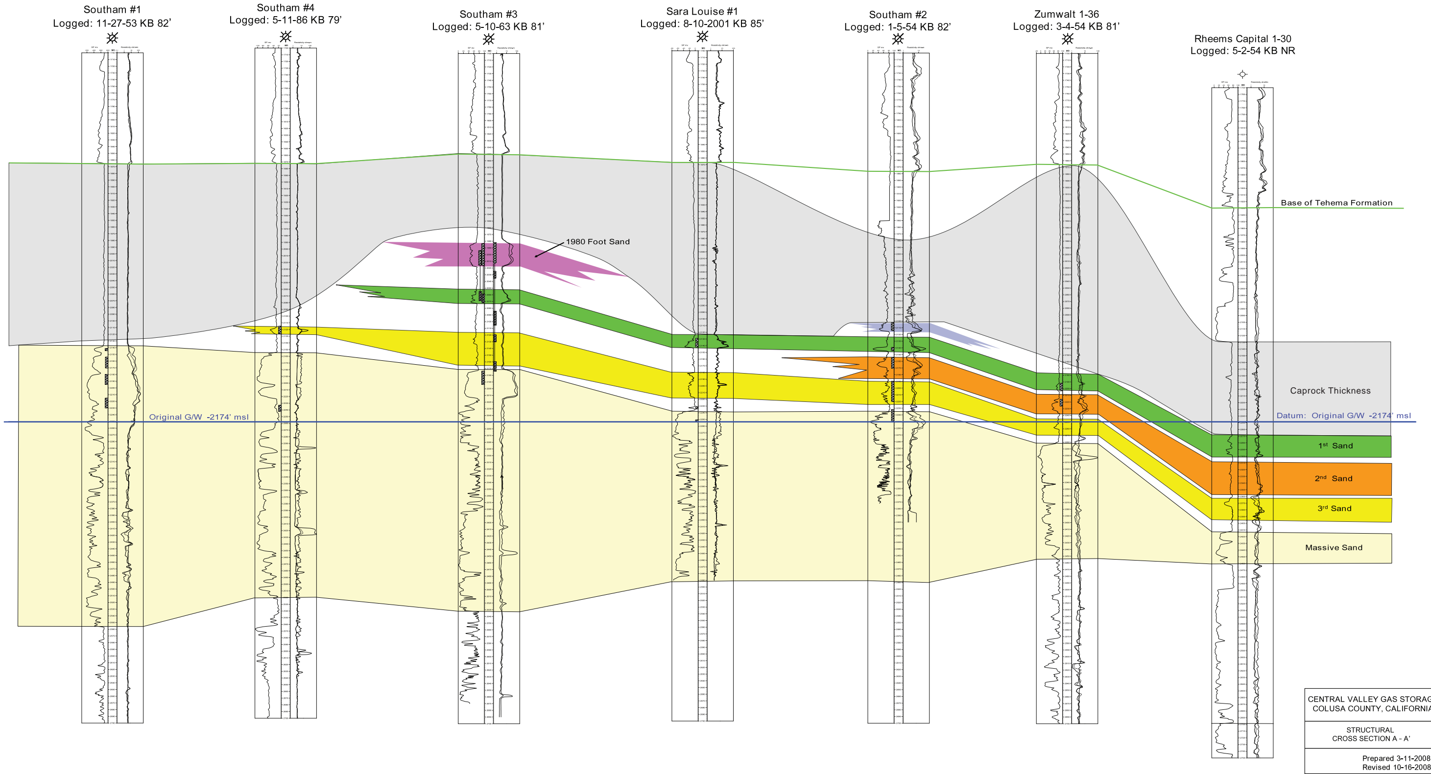
FIGURE 4-4 Cross Section of the Princeton Gas Field
