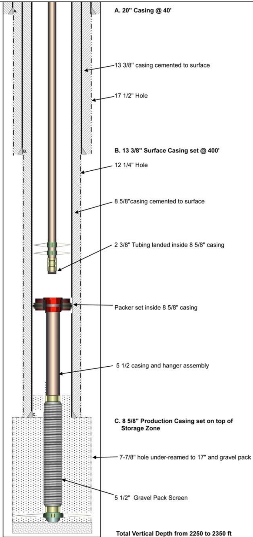
FIGURE 4-7 Well-bore Completion Diagram
