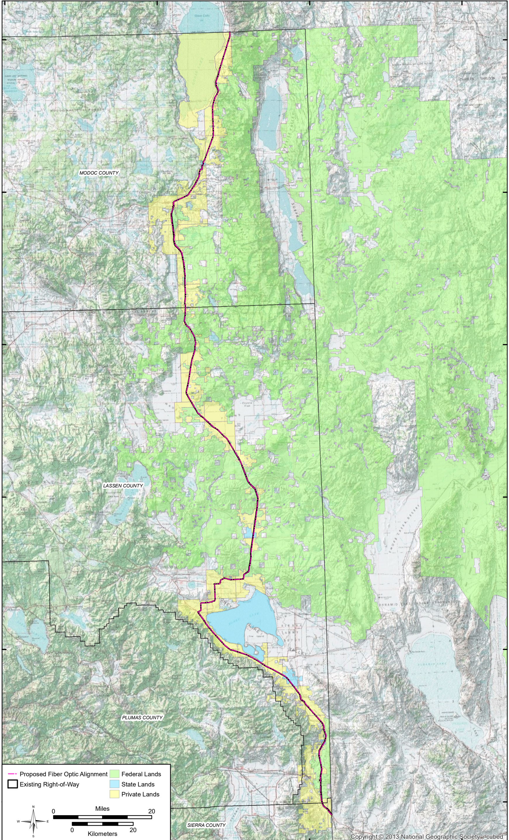
Figure 1. Zayo Fiber Optic Alignment and Right-of-Way (ver. 6/14/19).
