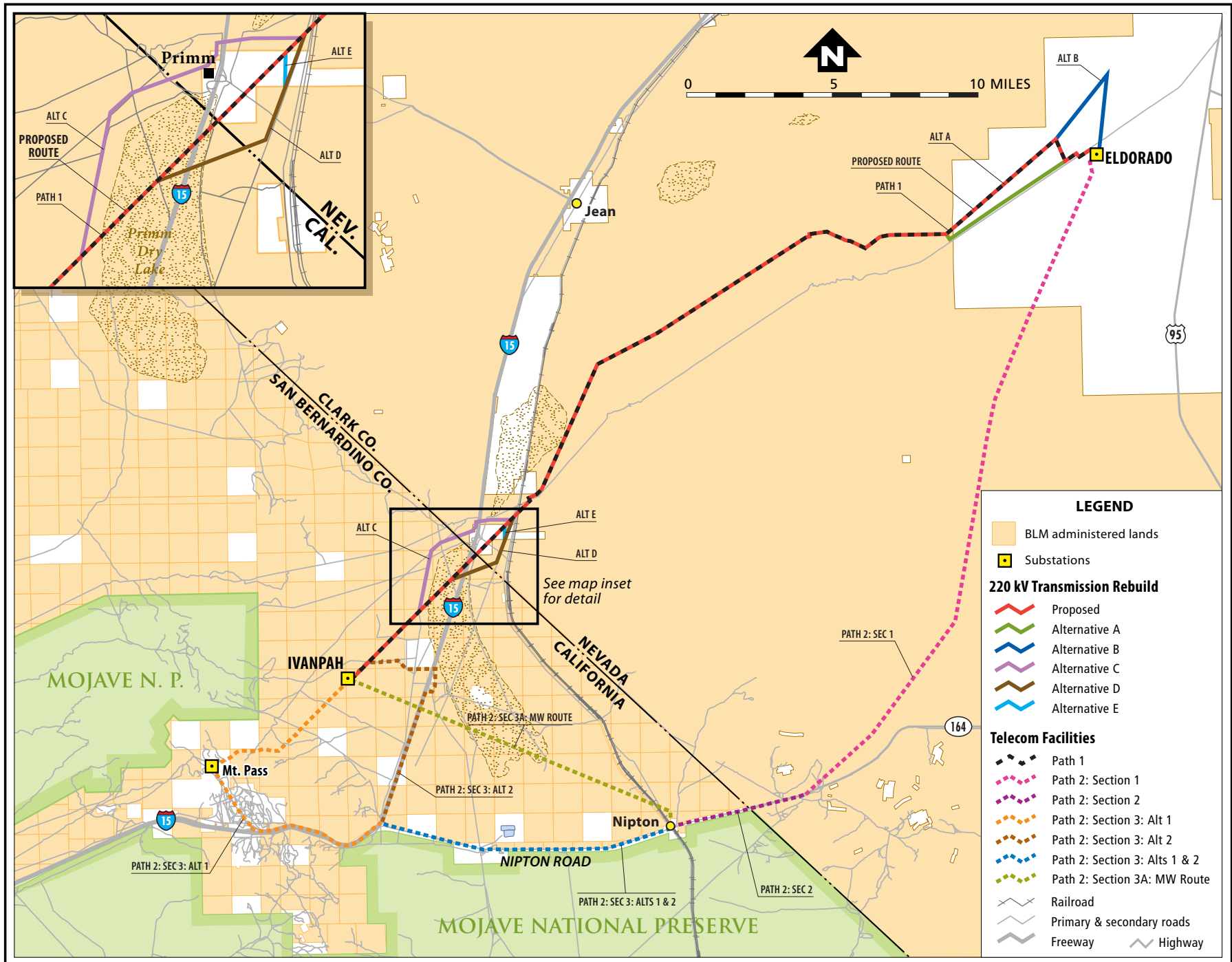
Figure ES-1 Components of the Ivanpah to Eldorado Transmission Project San Bernardino County, California and Clark County, Nevada
