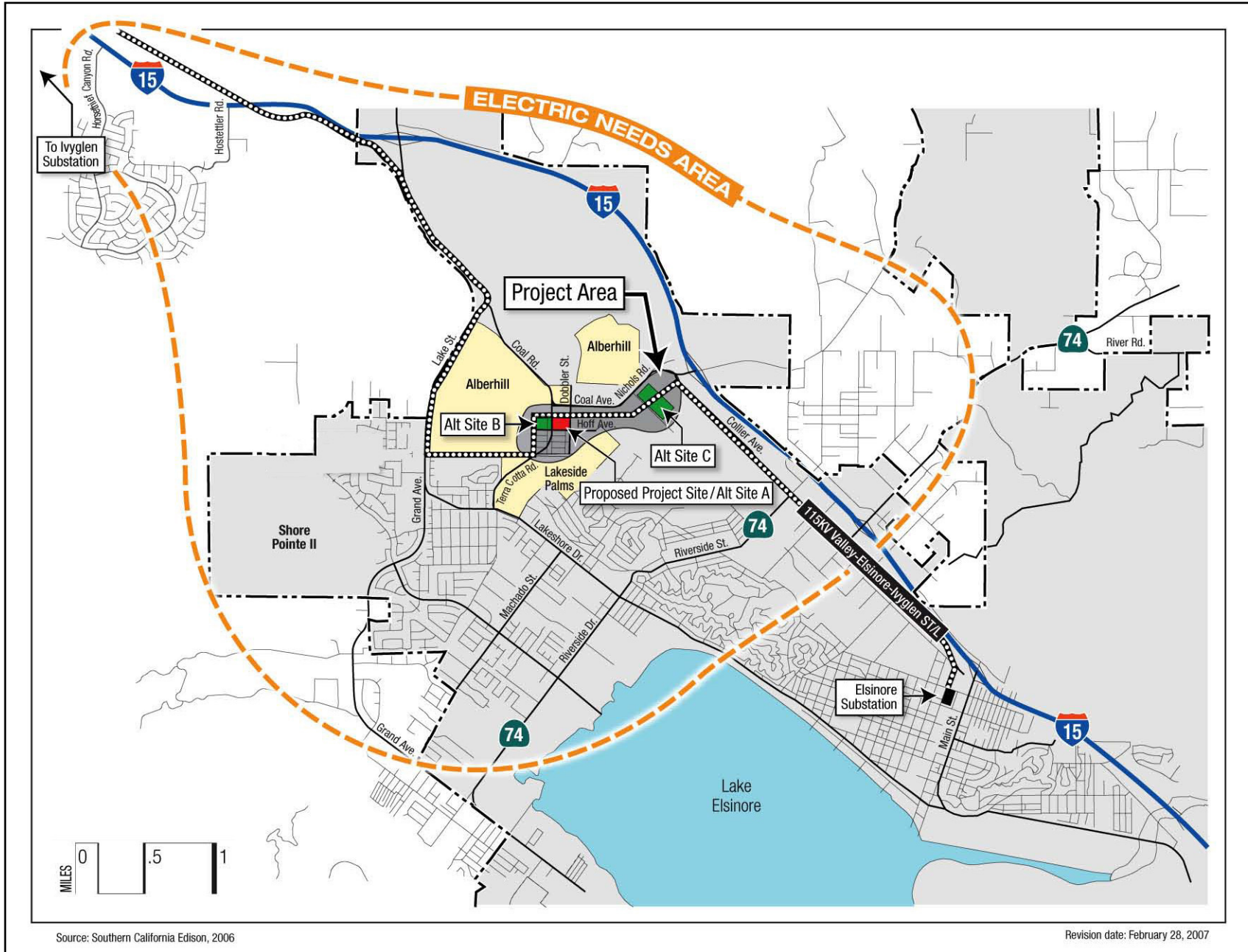
Figure A.1-2 Fogarty Electrical Needs Area
