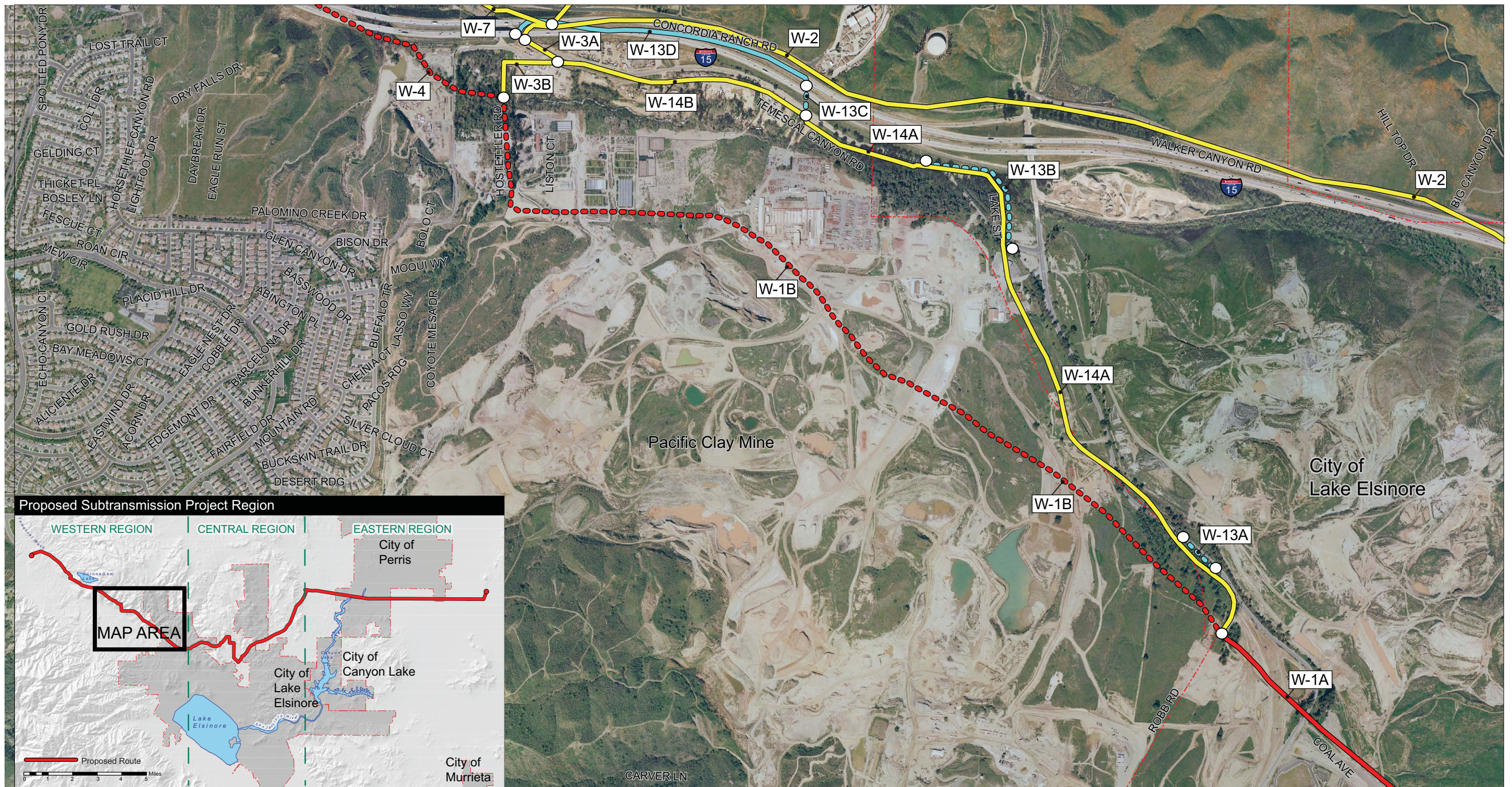
Figure C.2-7 Proposed Subtransmission and Alternative Route Segments
