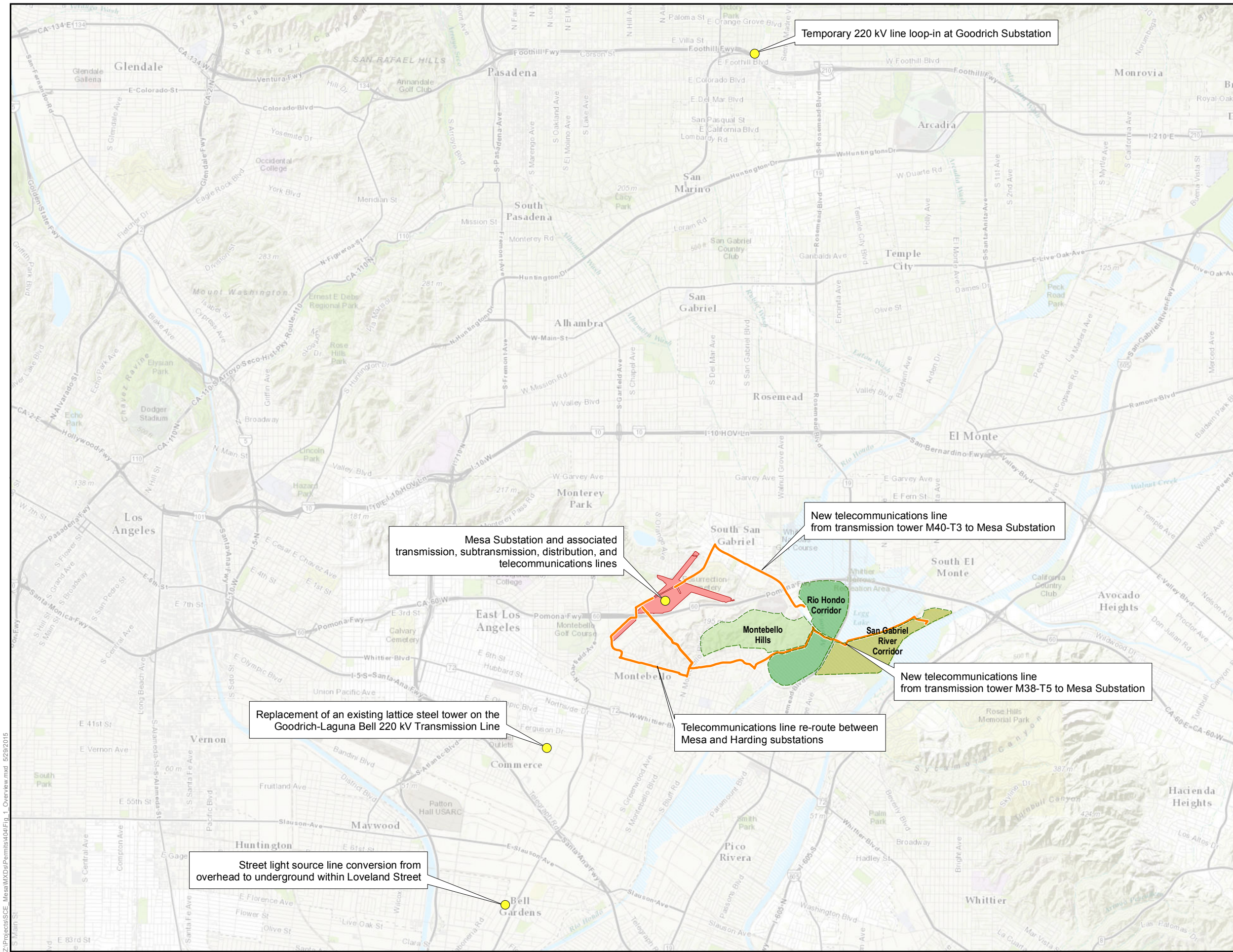
Figure 1: Project Components Overview Map Mesa 500 kV Substation Project
