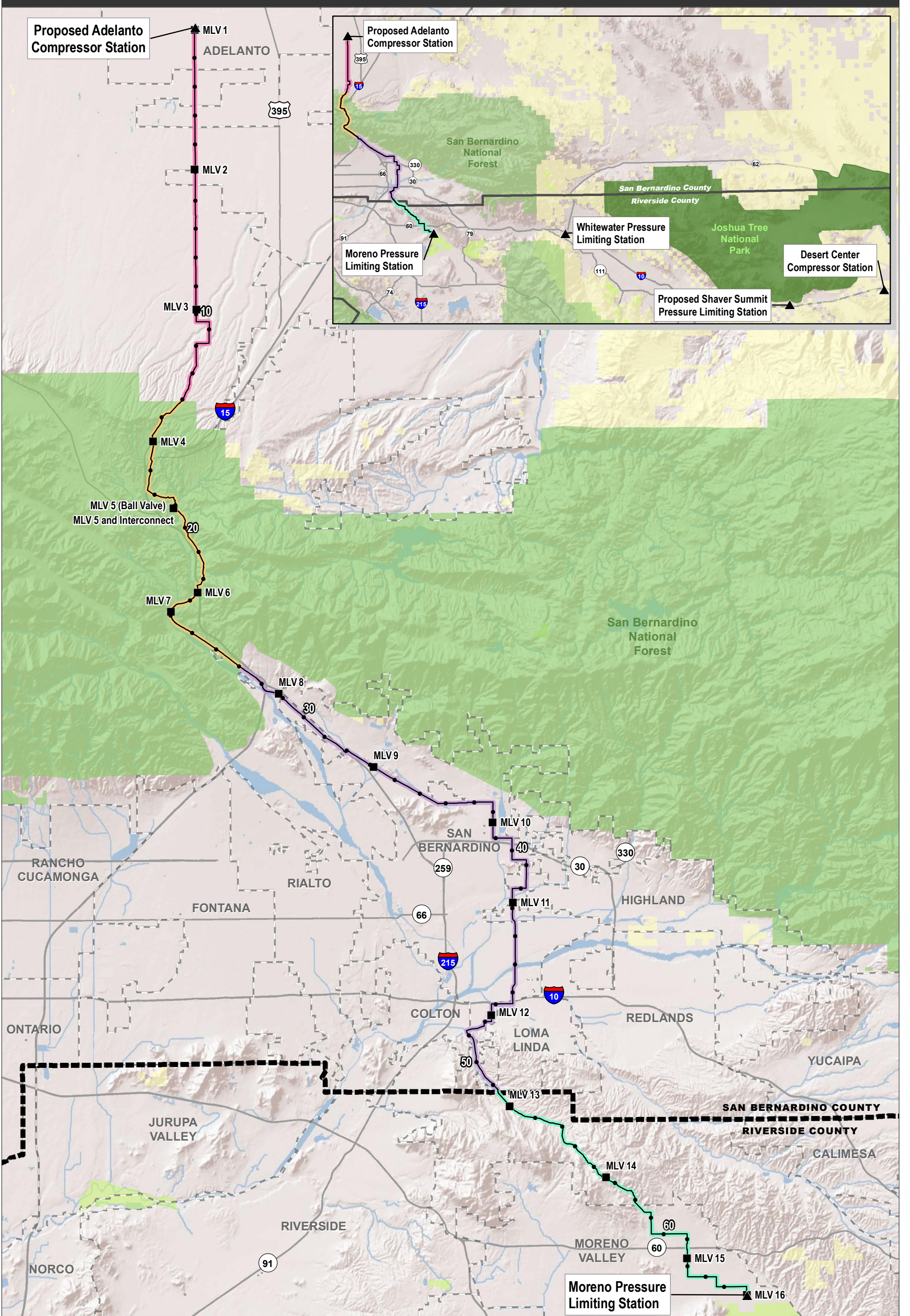
FIGURE 1 PROJECT OVERVIEW NORTH SOUTH PROJECT
