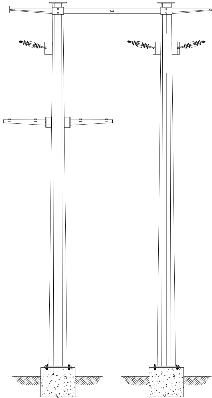
TYPICAL PROPOSED 138 kV DEADEND SINGLE CIRCUIT TUBULAR STEEL POLE H-FRAME STRUCTURE
