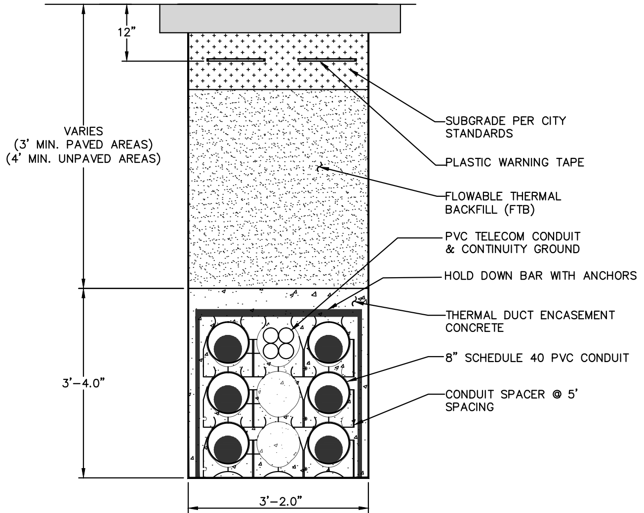
STANDARD CONDUIT PACKAGE NOT TO SCALE
