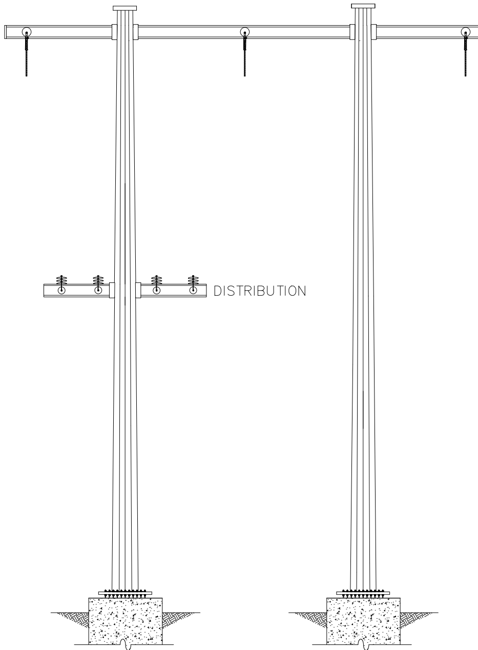
TYPICAL PROPOSED 138 kV SINGLE CIRCUIT D.E. STEEL H-FRAME WITH DISTRIBUTION UNDERBUILD
