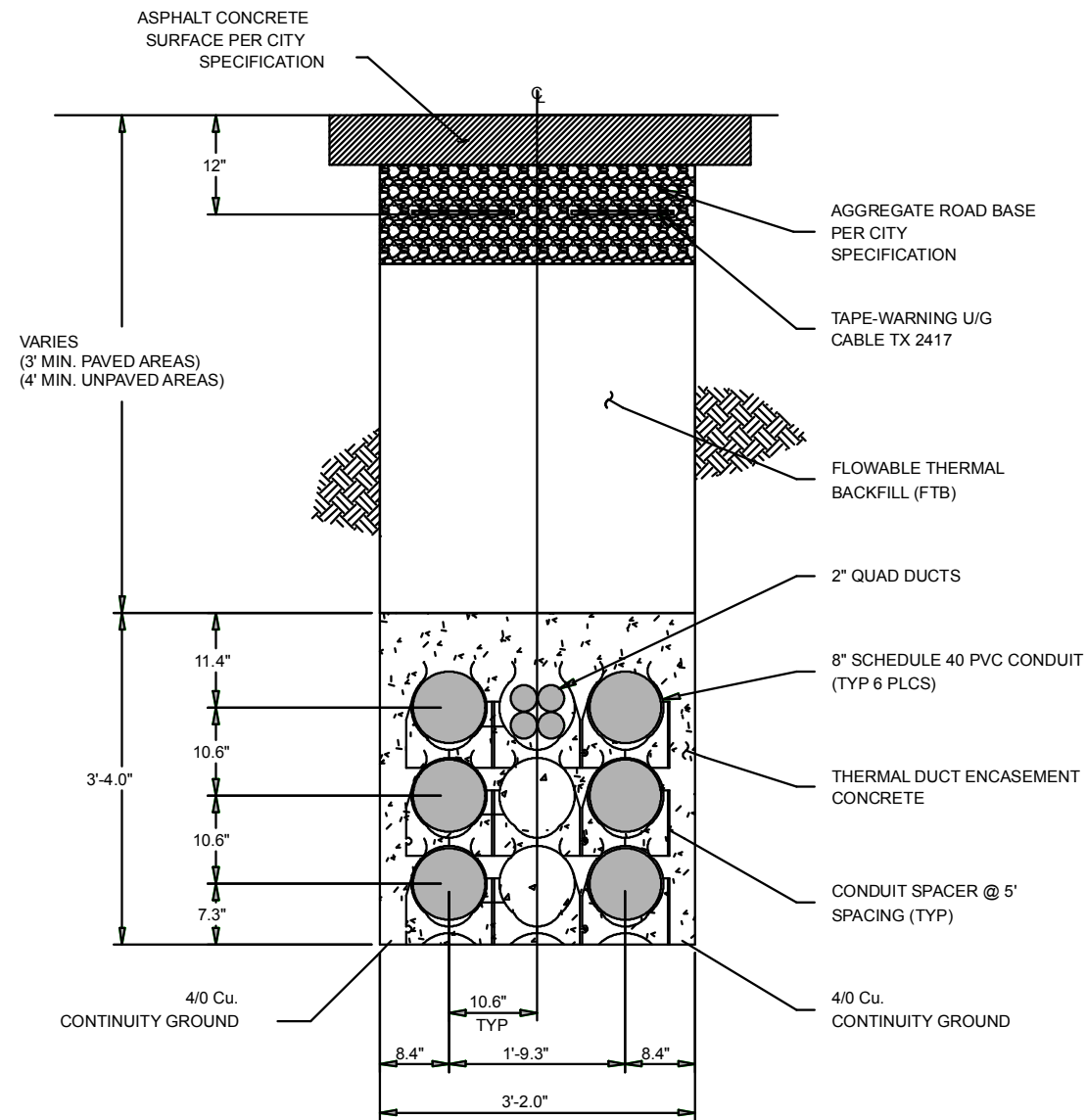
TYPICAL 230kV DOUBLE CIRCUIT DUCT BANK FIGURE 1.2 NOT TO SCALE
