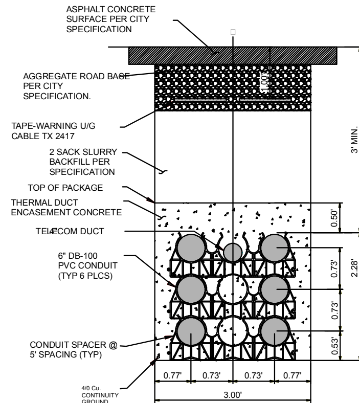
TYPICAL 69kV DOUBLE CIRCUIT DUCT BANK FIGURE 1.2 NOT TO SCALE
