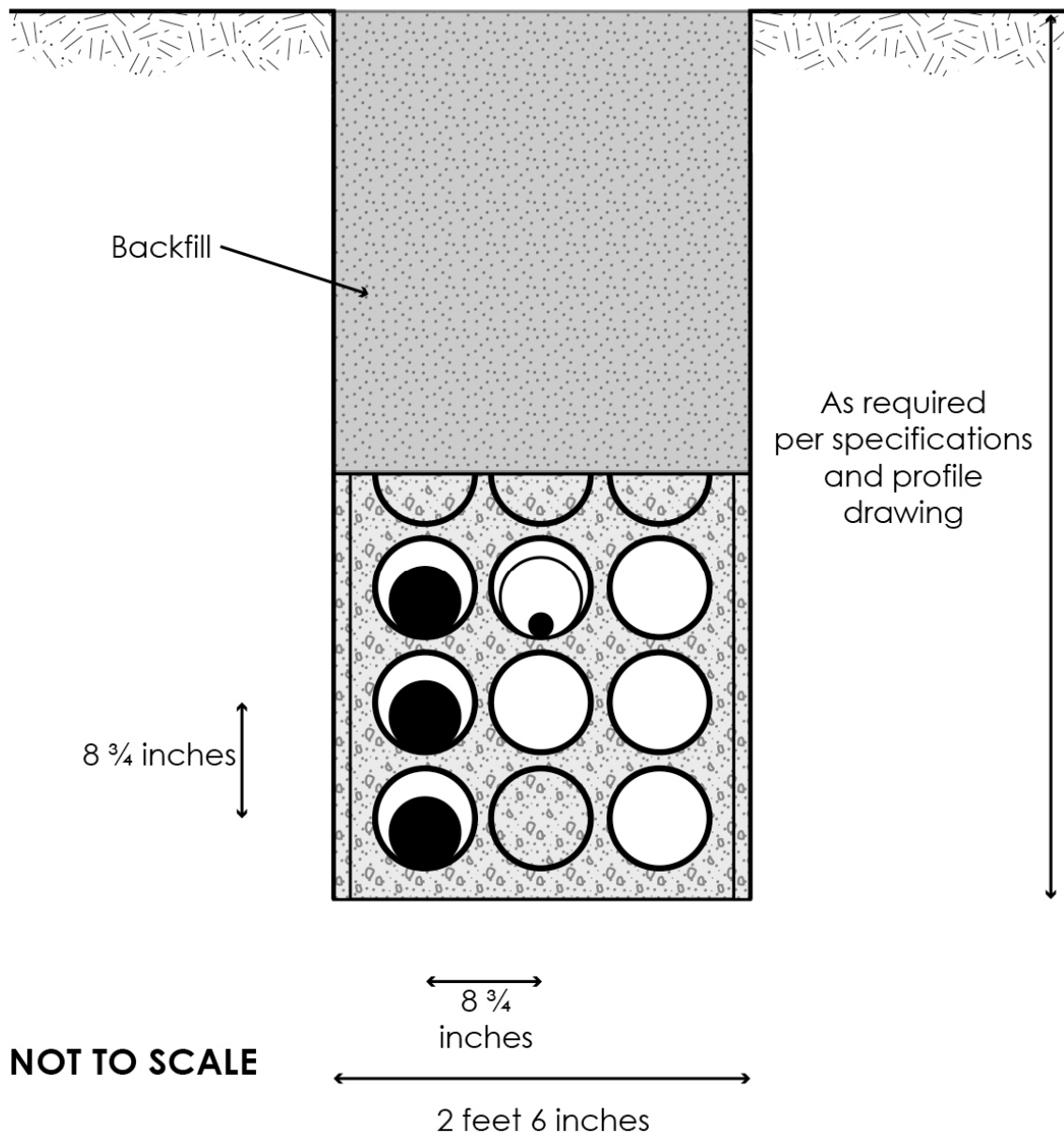
Figure 2.6-6 Diagram of Proposed 69-kV Duct Bank
