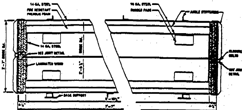
SECTION DOT SPECIFICATION 21PF-1A OVERPACK
