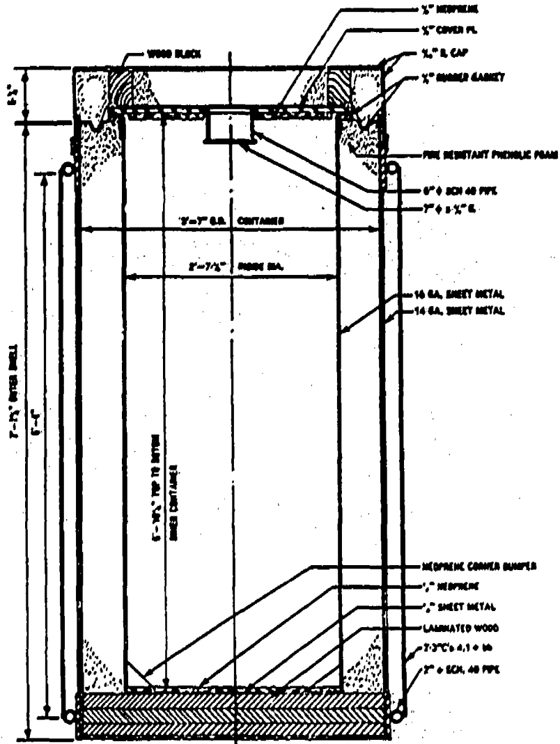
(c) Specification-21PF-2 (end loading overpack),
