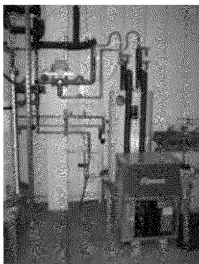
Figure 3: Water Tempering System
