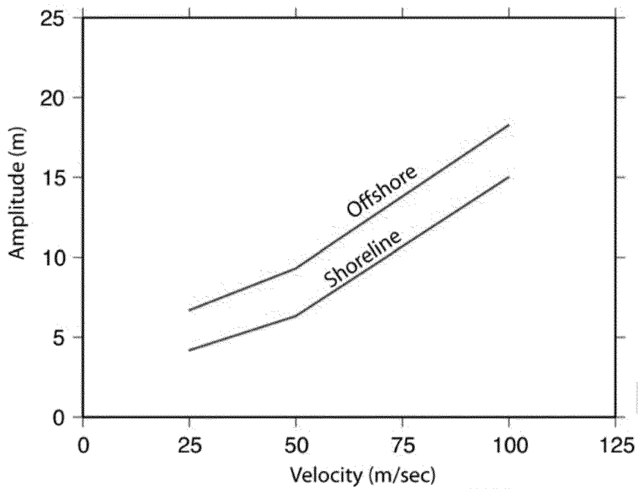
FIGURE A2-3 RUNUP HEIGHT AS A FUNCTION OF SLIDE VELOCITY FOR A SUBMARINE LANDSLIDE..... 23
