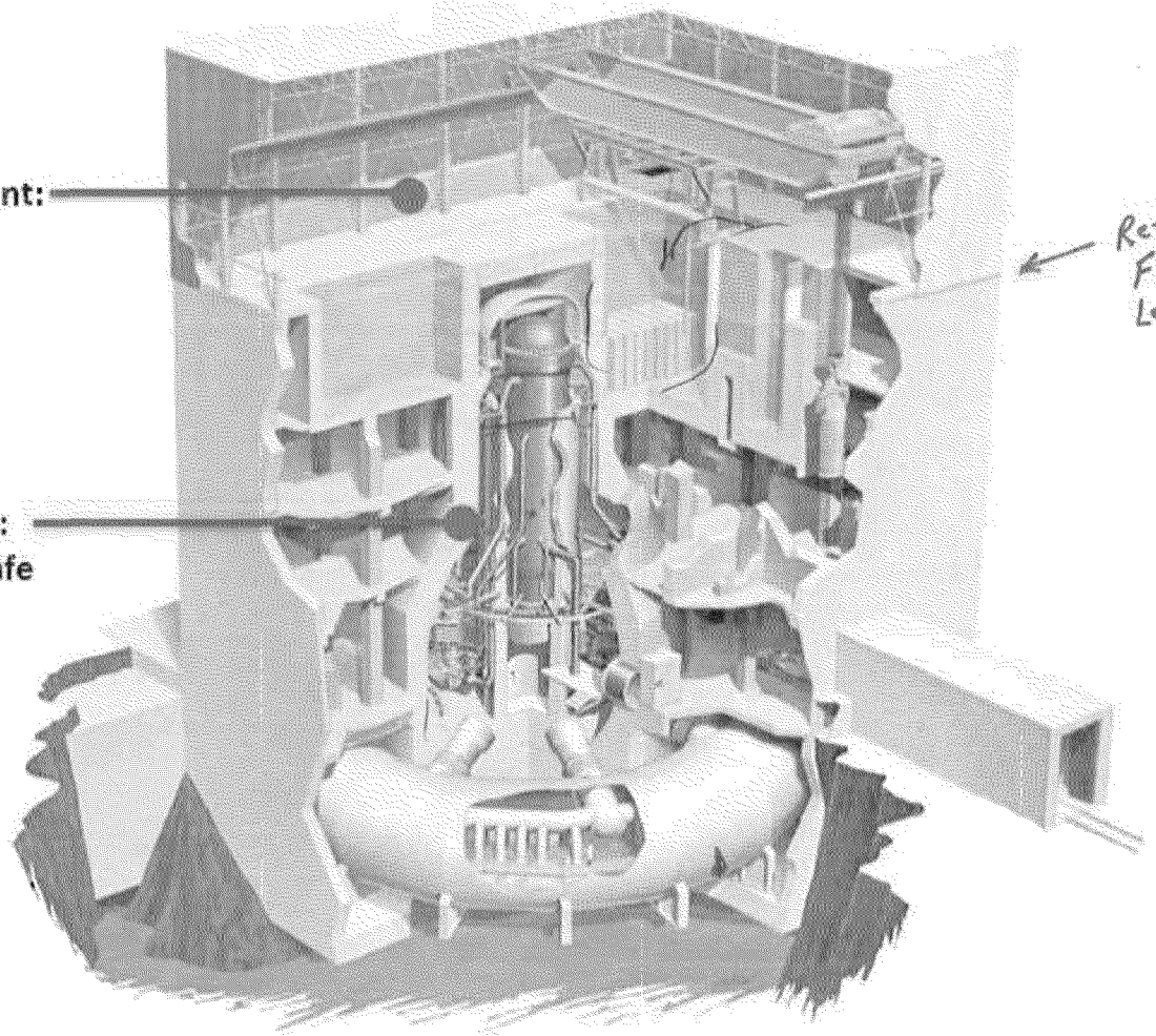
Boiling Water Reactor Design
