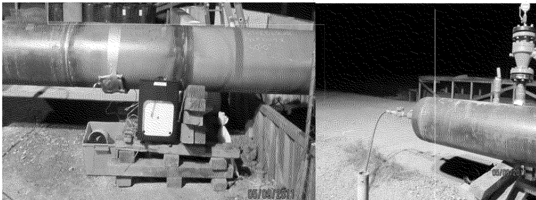
Test Head and Valving with Unrestrained Temperature Recorder
