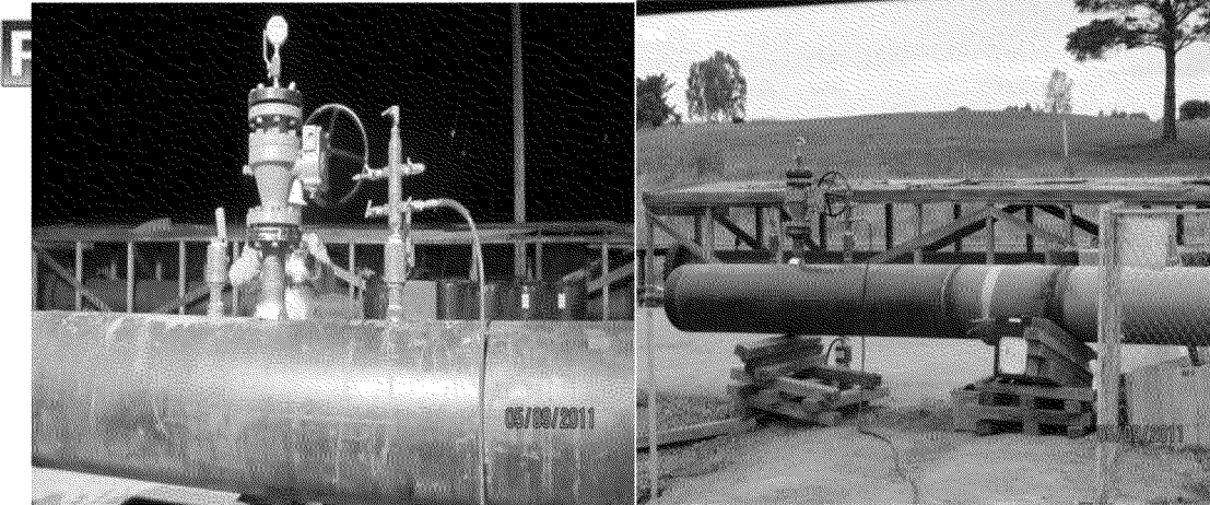
Test Head and Valving with Unrestrained Temperature Recorder
