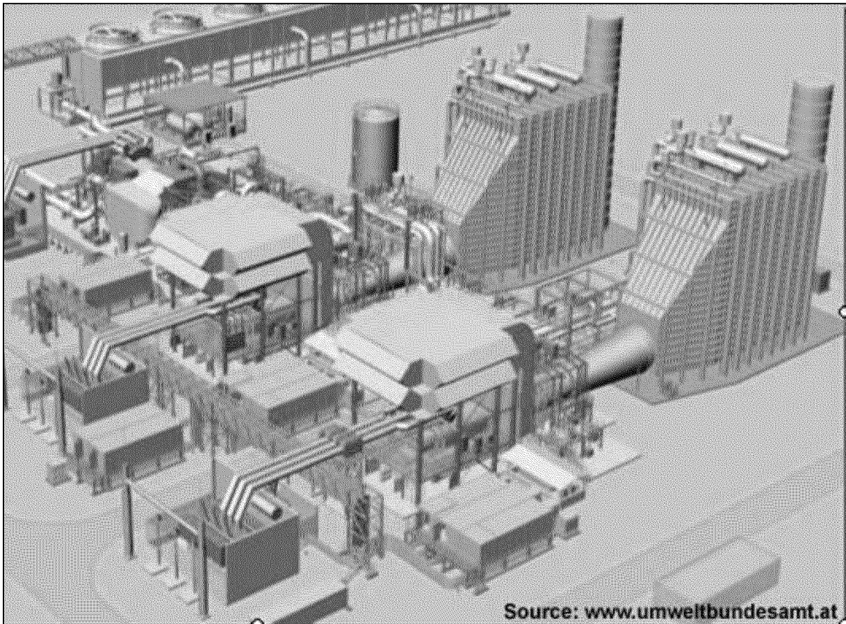
Figure C-4: Combined Cycle Power Plant General Arrangement
