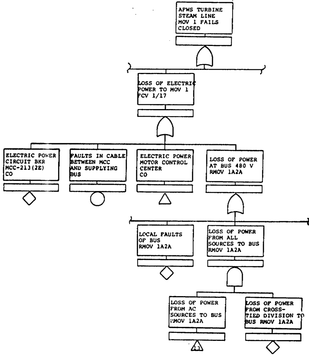
Figure 4.1. Portion of AFWS Fault Tree.
