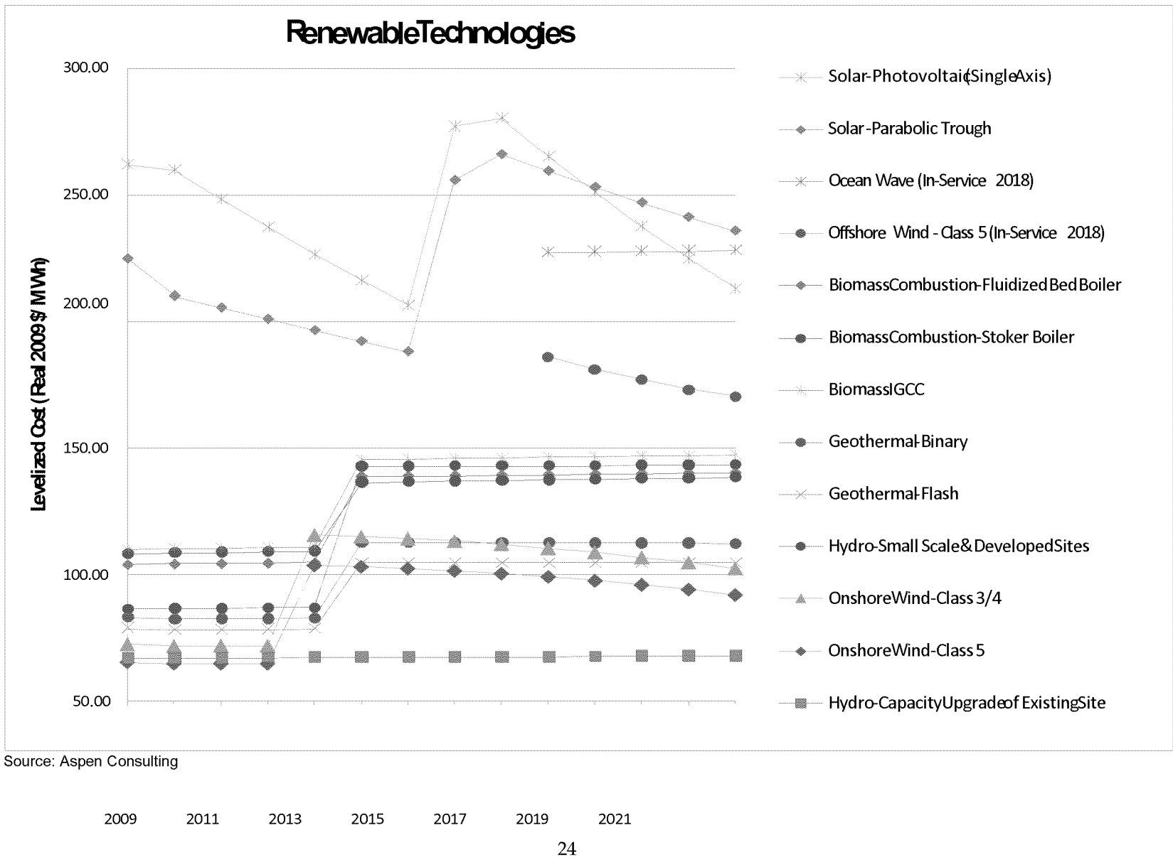
Figure 10: Average Merchant Levelized Cost Trend for Renewable Technologies
