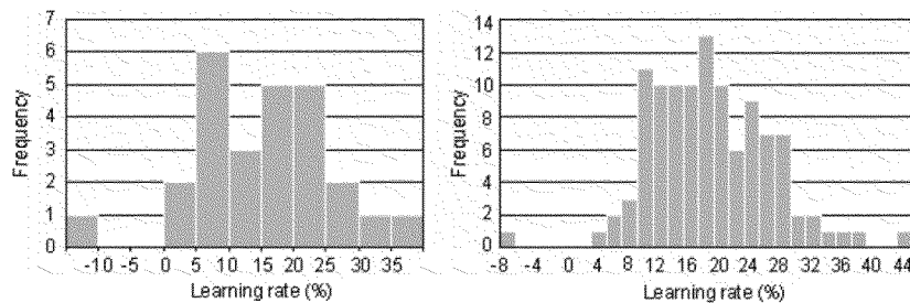
Fig. 2. Distribution of learning rates in Table 1 (left panel) and as observed in 22 "eld studies (right panel) (Dutton and Thomas, 1984).
