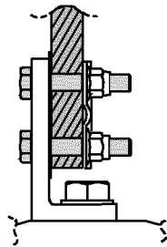
Figure 8.2.1 Correct installation
