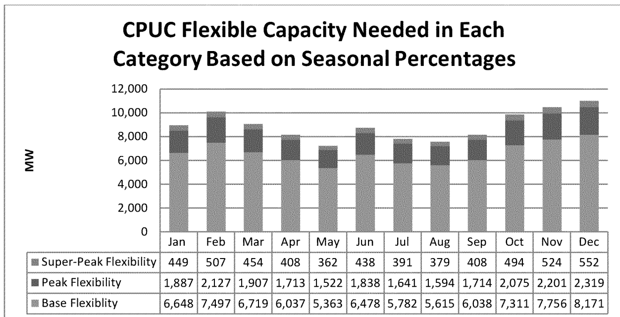
Figure 6: CPUC Flexible Capacity Need in Each Category for 2015
