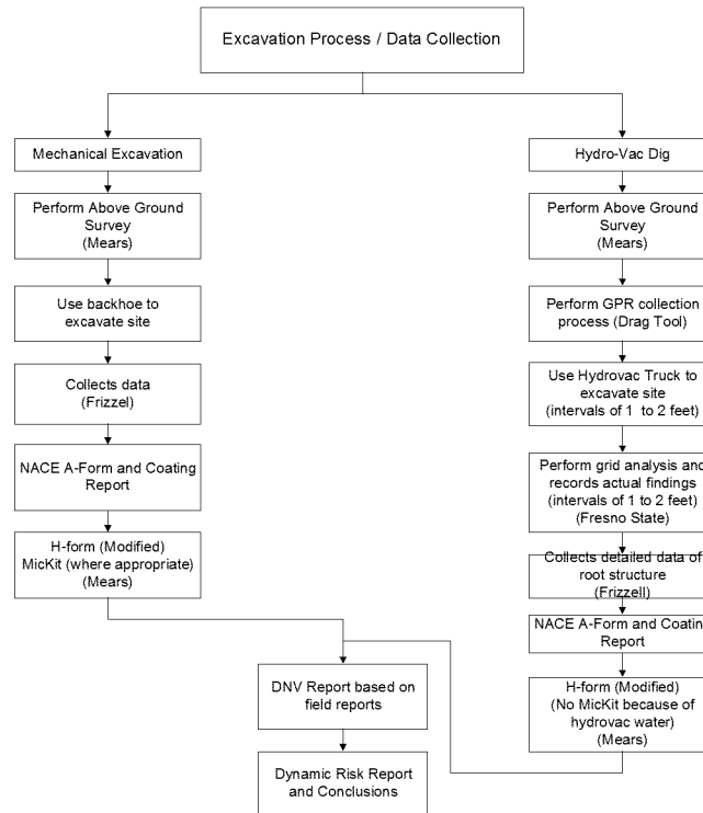
Figure 1. Excavation Process
