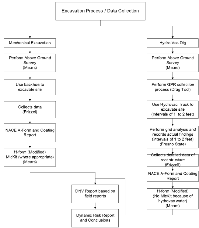
Figure 1. Excavation Process
