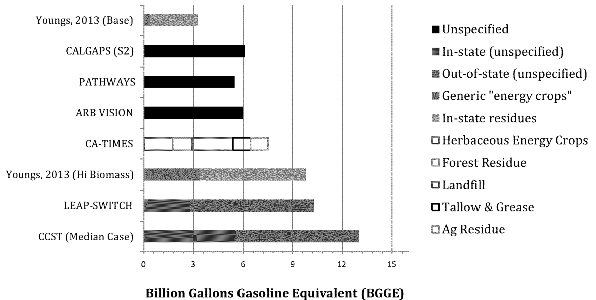
Figure 5. Maximum assumed biofuel volumes in 2050 across models/scenarios.
