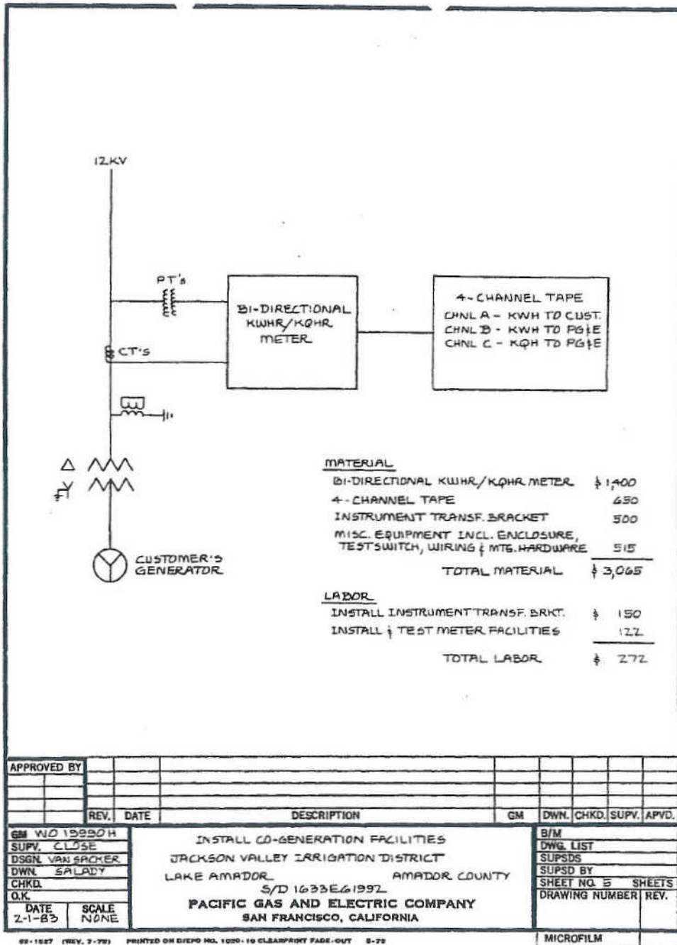
Single Line Diagram
