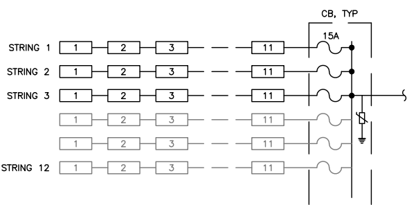
DETAIL OF SOLAR PANELS AND COMBINER BOX FOR SUNTECH 280W PANEL
