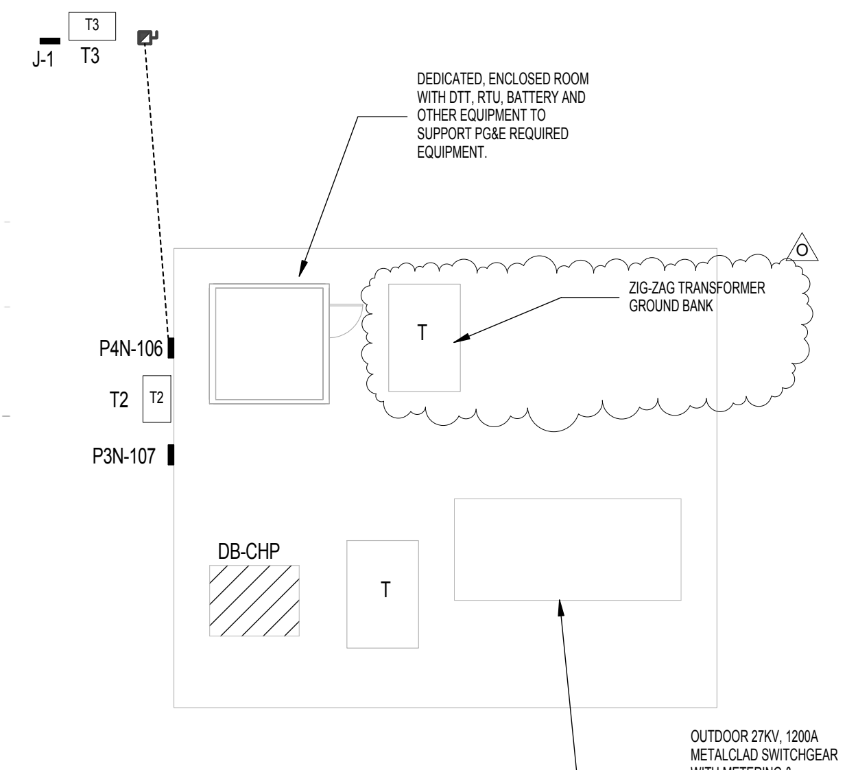
2 ENLARGED ELECTRICAL PLAN 3/32" = 1'-0"
