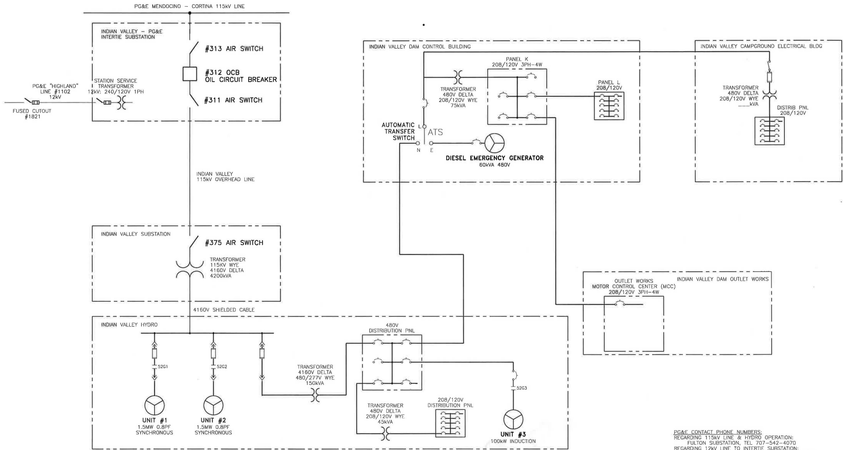
INDIAN VALLEY DAM ELECTRICAL ONE-LINE SCHEMATIC
