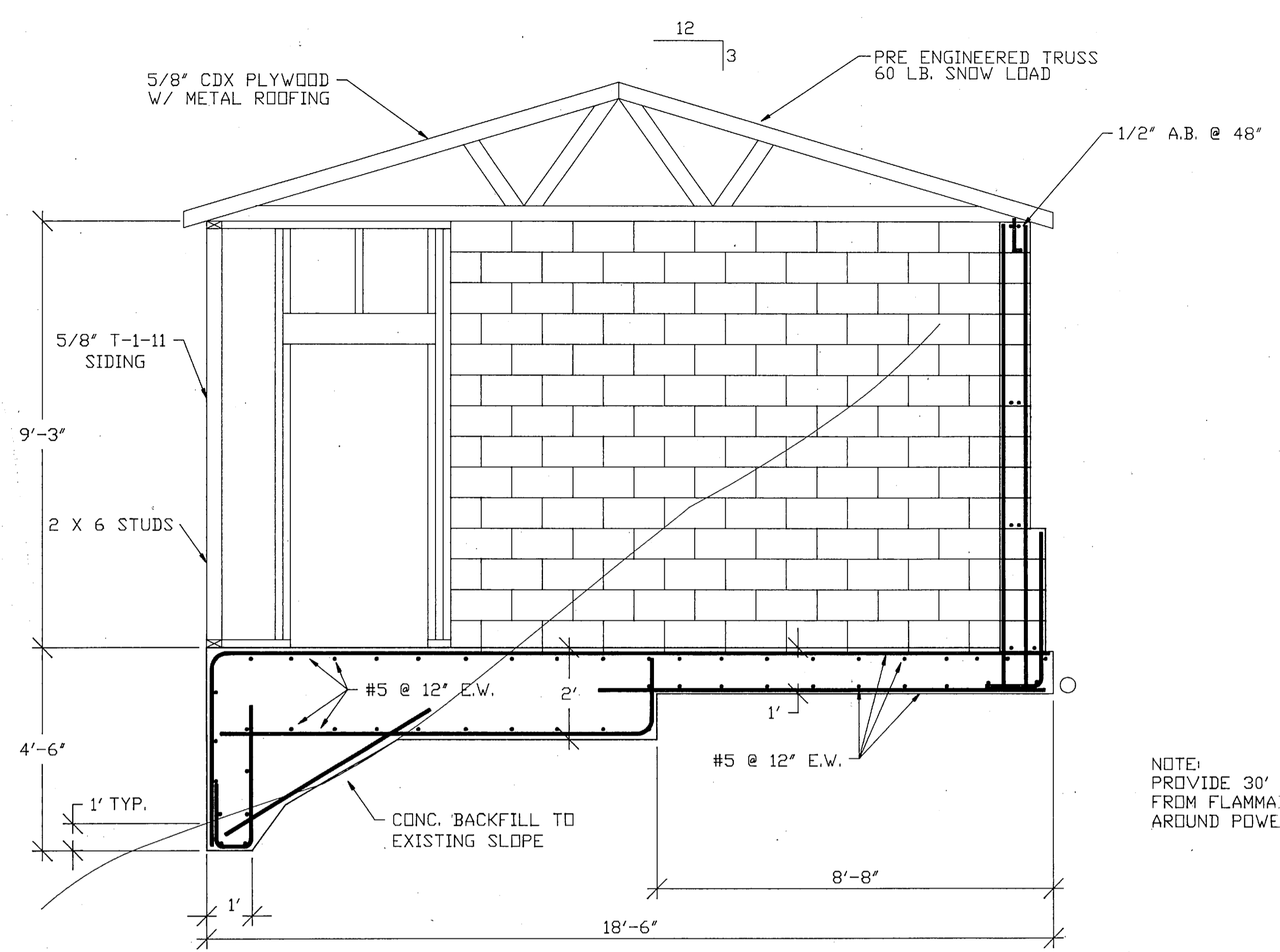
DETAIL A
