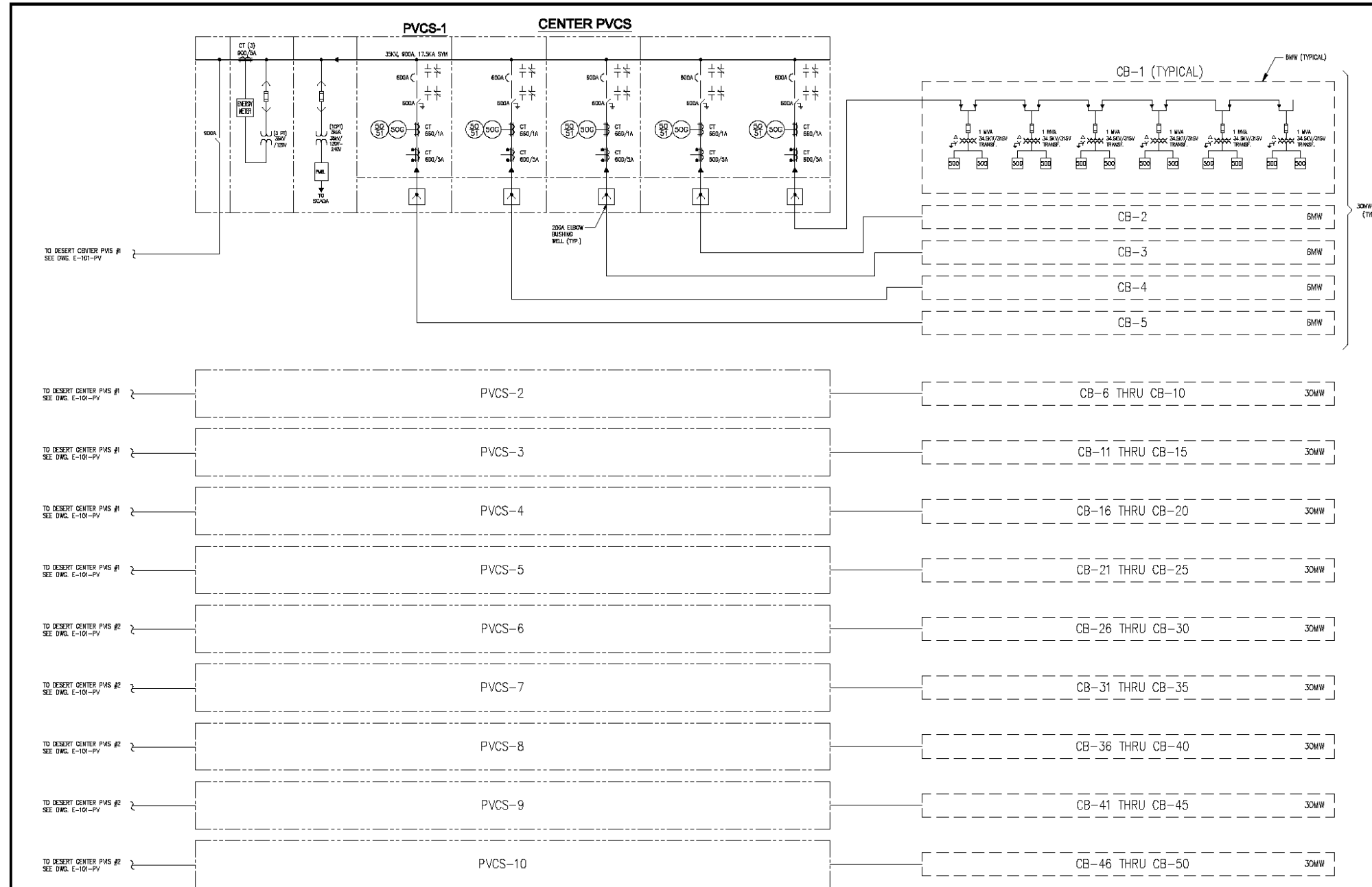
CENTER PVCS MAIN ONE LINE DIAGRAM (SHT 3) - 300MW ac SYSTEM SCALE: N.T.S.
