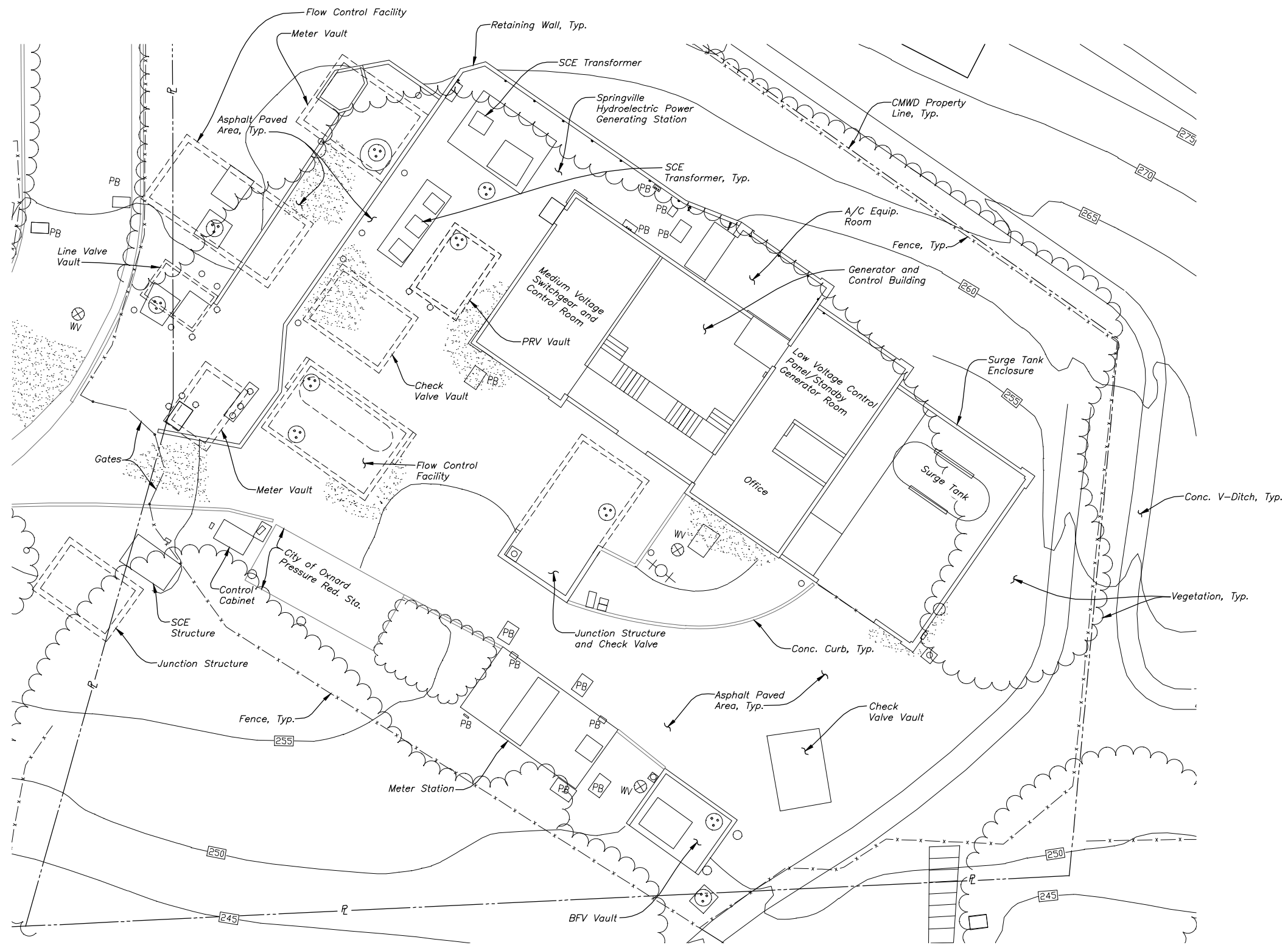
HYDROELECTRIC POWER STATION GENERAL LAYOUT PLAN SCALE: 1 IN. = 10 FT.
