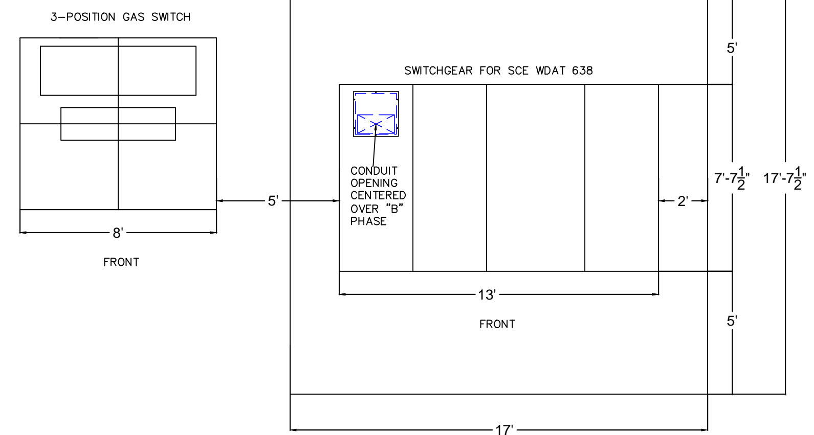
SWITCHGEAR PLAN VIEW SCALE: 1/4"=1' @ 24" x 36"
