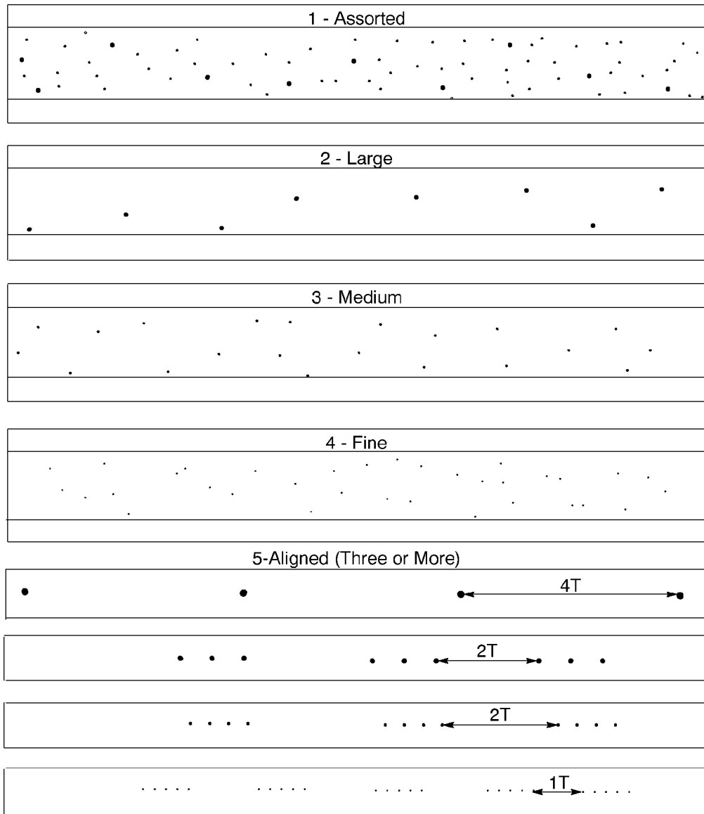
Figure 20 Maximum Distribution of Gas Pockets Wall Thickness, Over 1/2" to 1-1/4"
