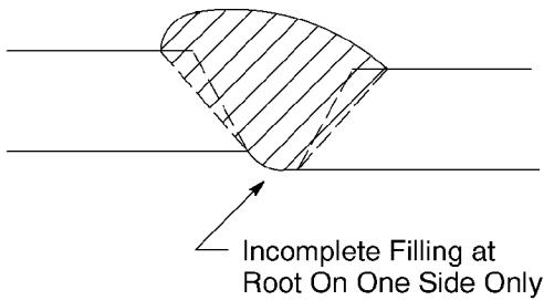
Figure 2 Inadequate Penetration Due to High-Low
