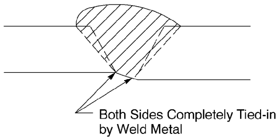
Figure 3 Penetration Adequate With High-Low Present
