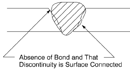
Figure 5 Incomplete Fusion at Root of Bead or Top of the Joint
