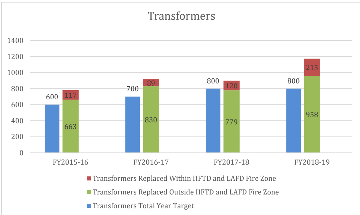
Graph 3: PSRP Transformer
