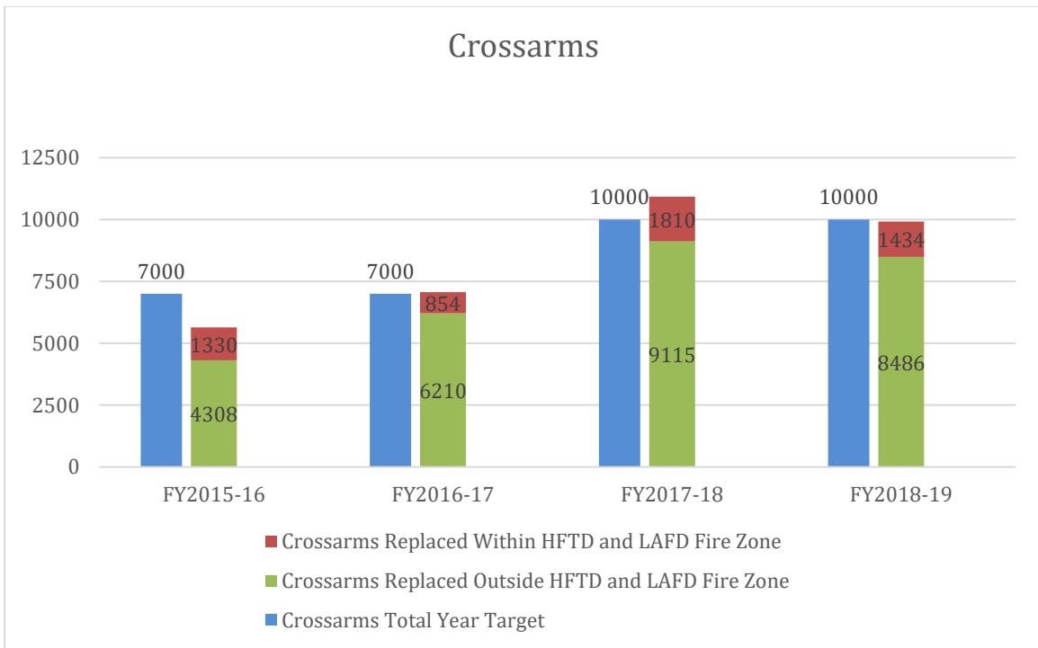
Graph 2: PSRP Crossarm
