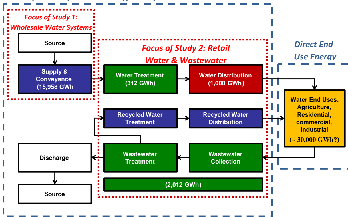
Figure E-1 – Water-Related Electricity Consumption by Segment of the Water Use Cycle 5 Indirect, or “Embedded” Energy (Upstream & Downstream of End Use) = Direct Energy Use by Water & Wastewater
