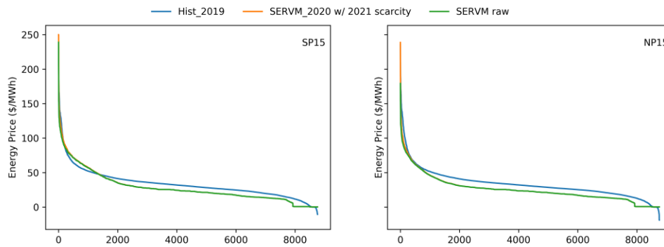
Figure 11. Impact of current year’s scarcity adjustment on raw SERVM prices relative to historical data
