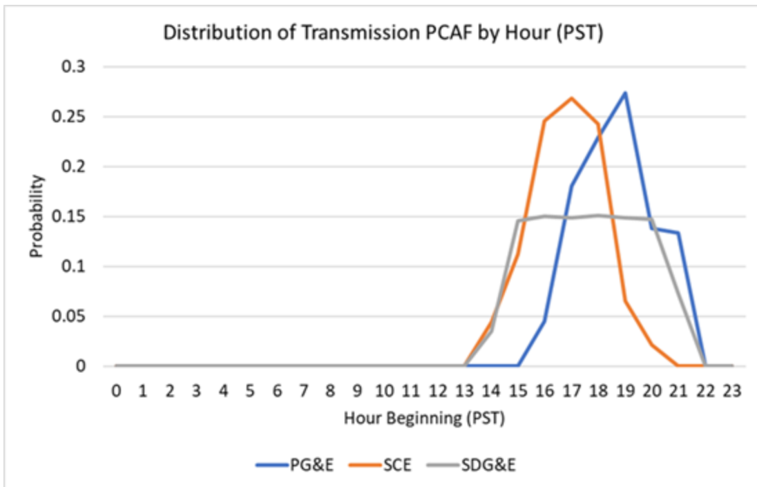
Figure 34- Transmission PCAF Allocators by IOU
