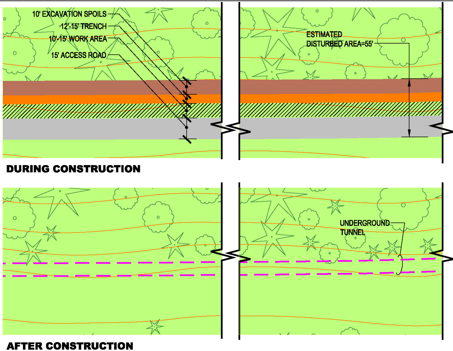
Figure 3.2-16 Underground Construction Cut/Cover Trenching Plan View
