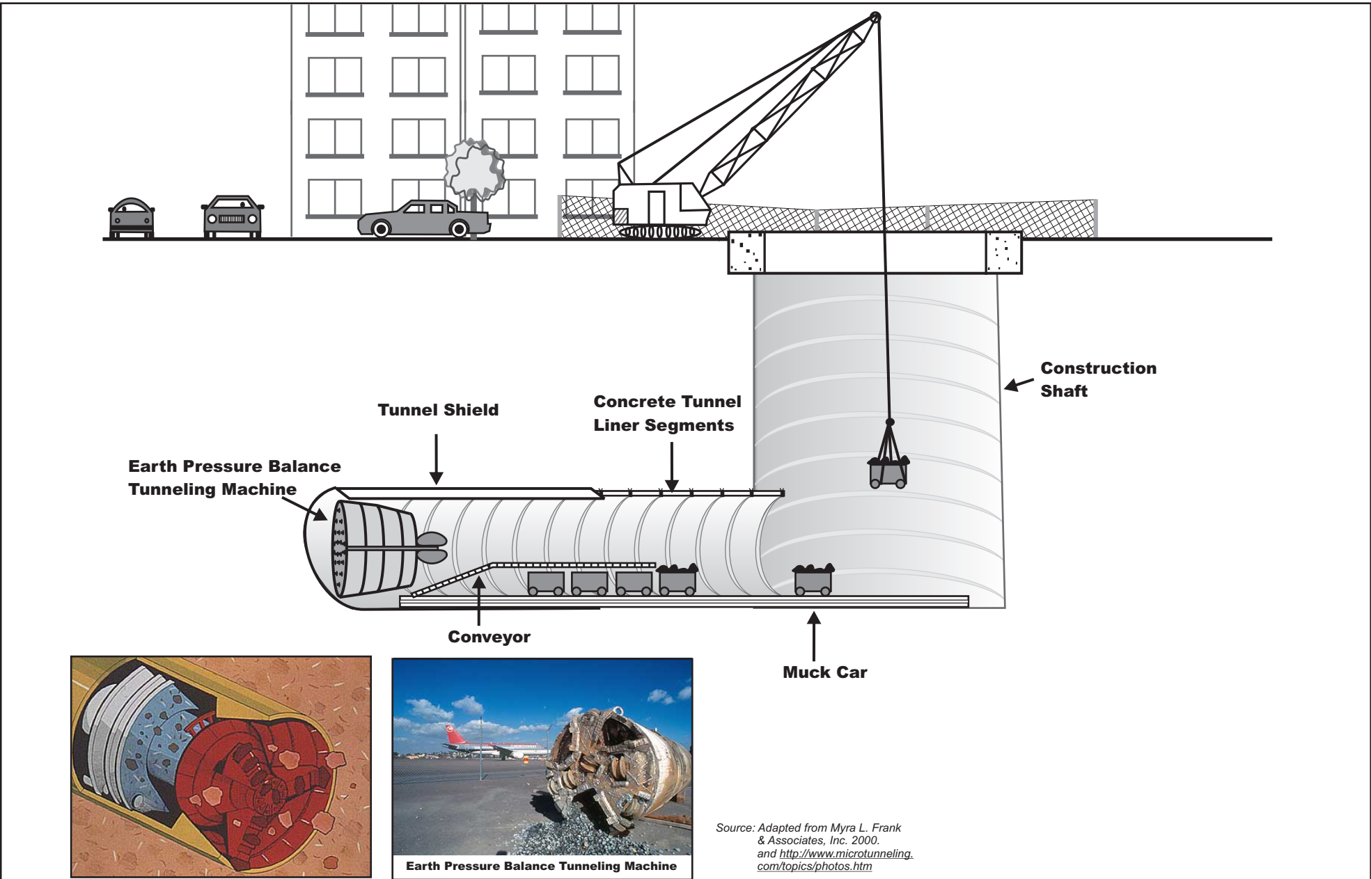
Figure 3.2-18 Typical Tunneling Operation
