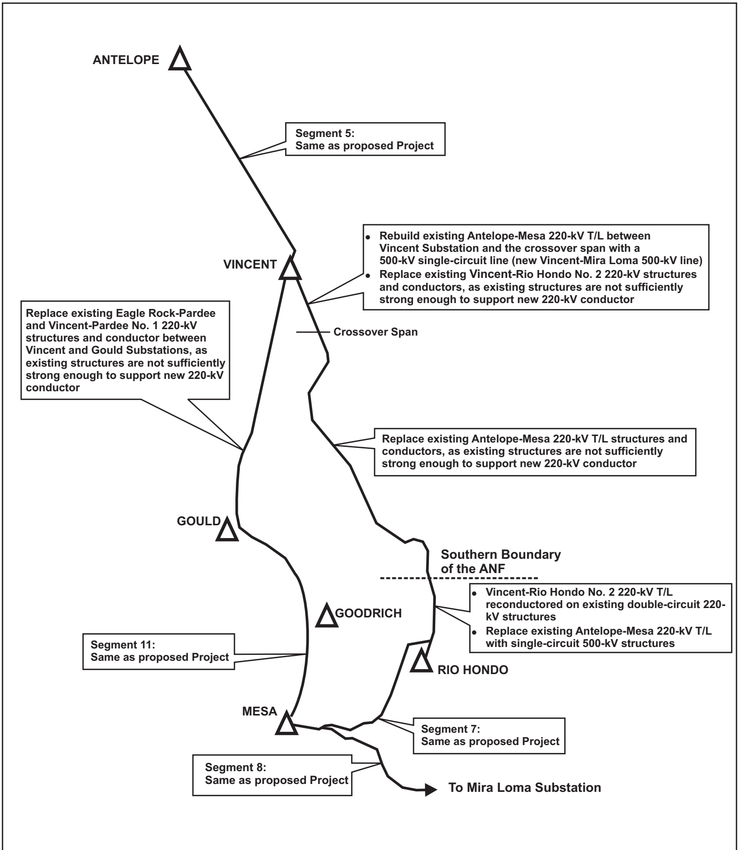
Figure 3.2-6 Minimize 500-kV Upgrades Alternative
