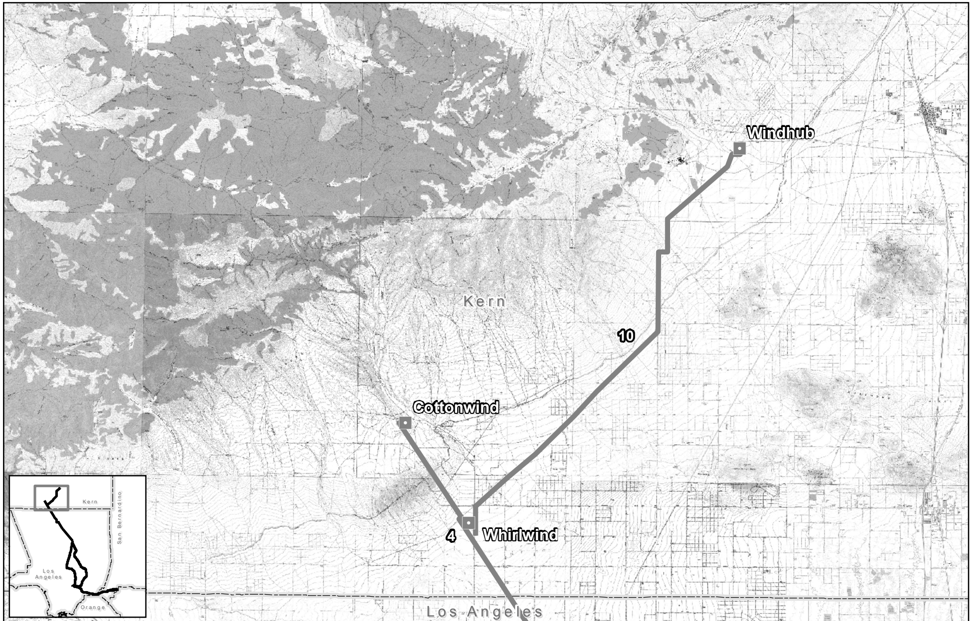
Figure 3.3-2 Windhub Substation to Cottonwind Substation to Whirlwind Substation Alternative
