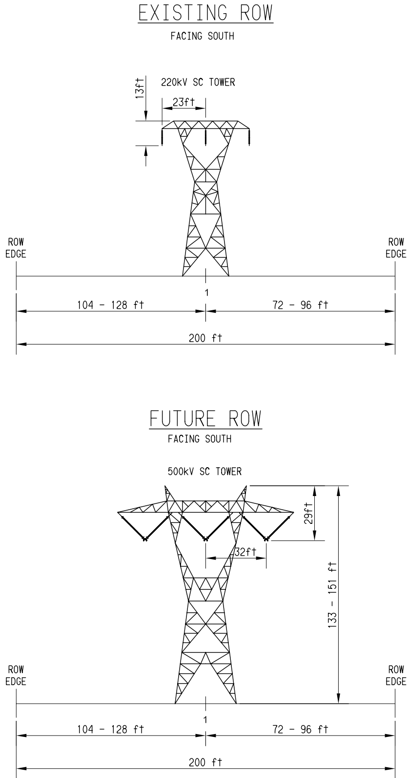
Figure 2.2-16 Segment 6 ROW Cross-Section (S6 MP 6.85 to S6 MP 7.75)
