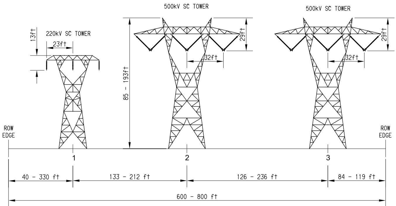
Figure 2.2-18 Segment 6 ROW Cross-Section (S6 MP 9.5 to S6 MP 26.9)
