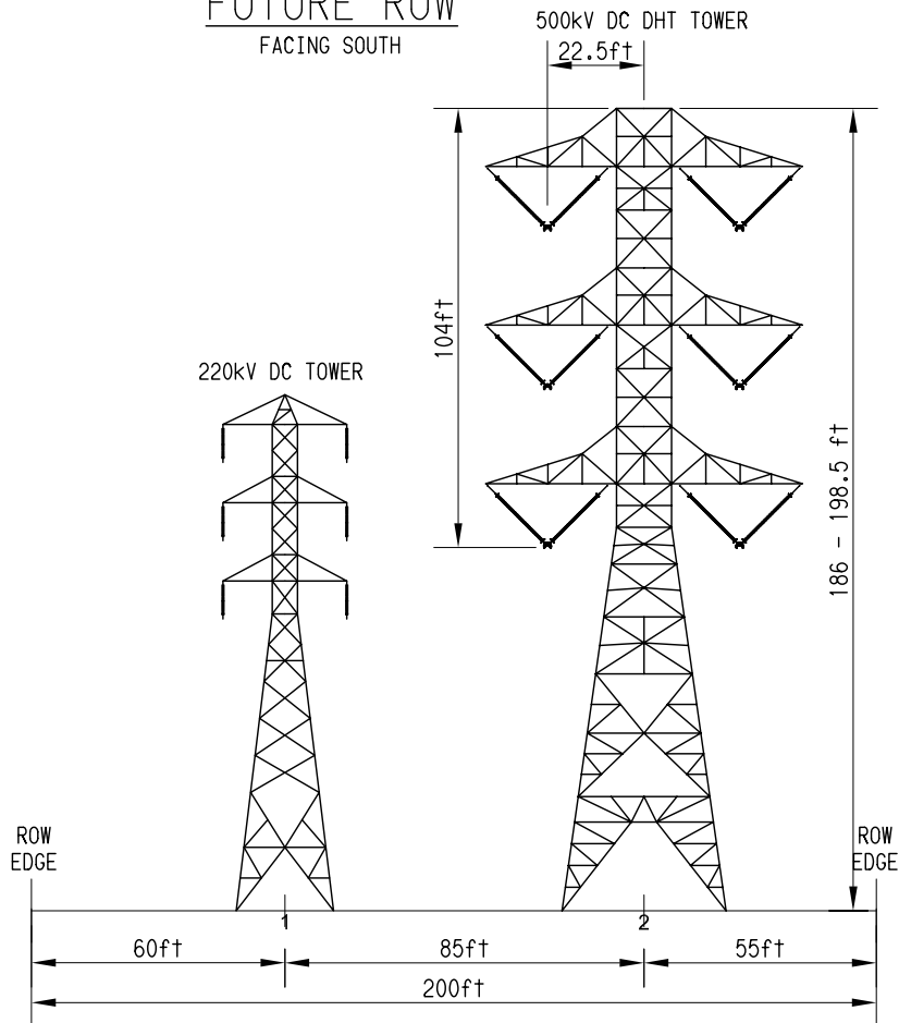
Figure 2.2-19 Segment 7 ROW Cross-Section (S7 MP 1.0 to S7 MP 1.2)
