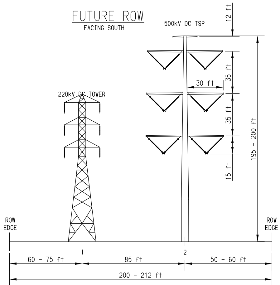
Figure 2.2-20 Segment 7 ROW Cross-Section (S7 MP 1.2 to S7 MP 1.7)
