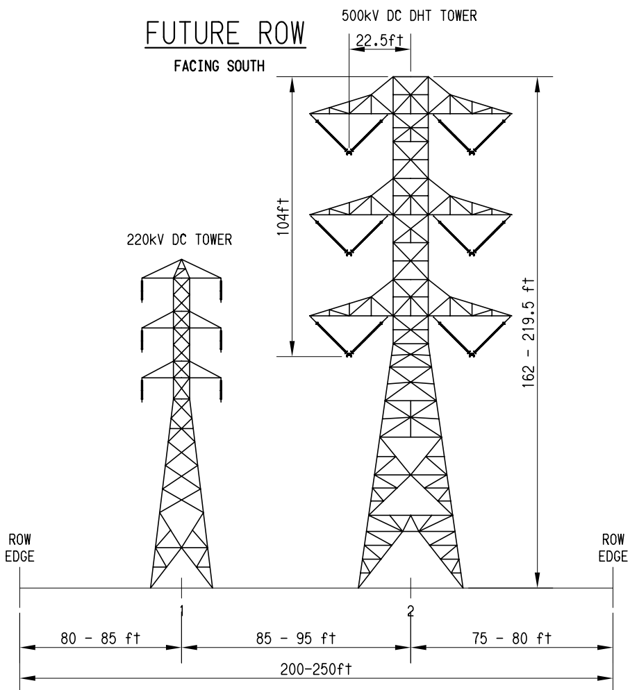
Figure 2.2-21 Segment 7 ROW Cross-Section (S7 MP 1.7 to S7 MP 4.3)
