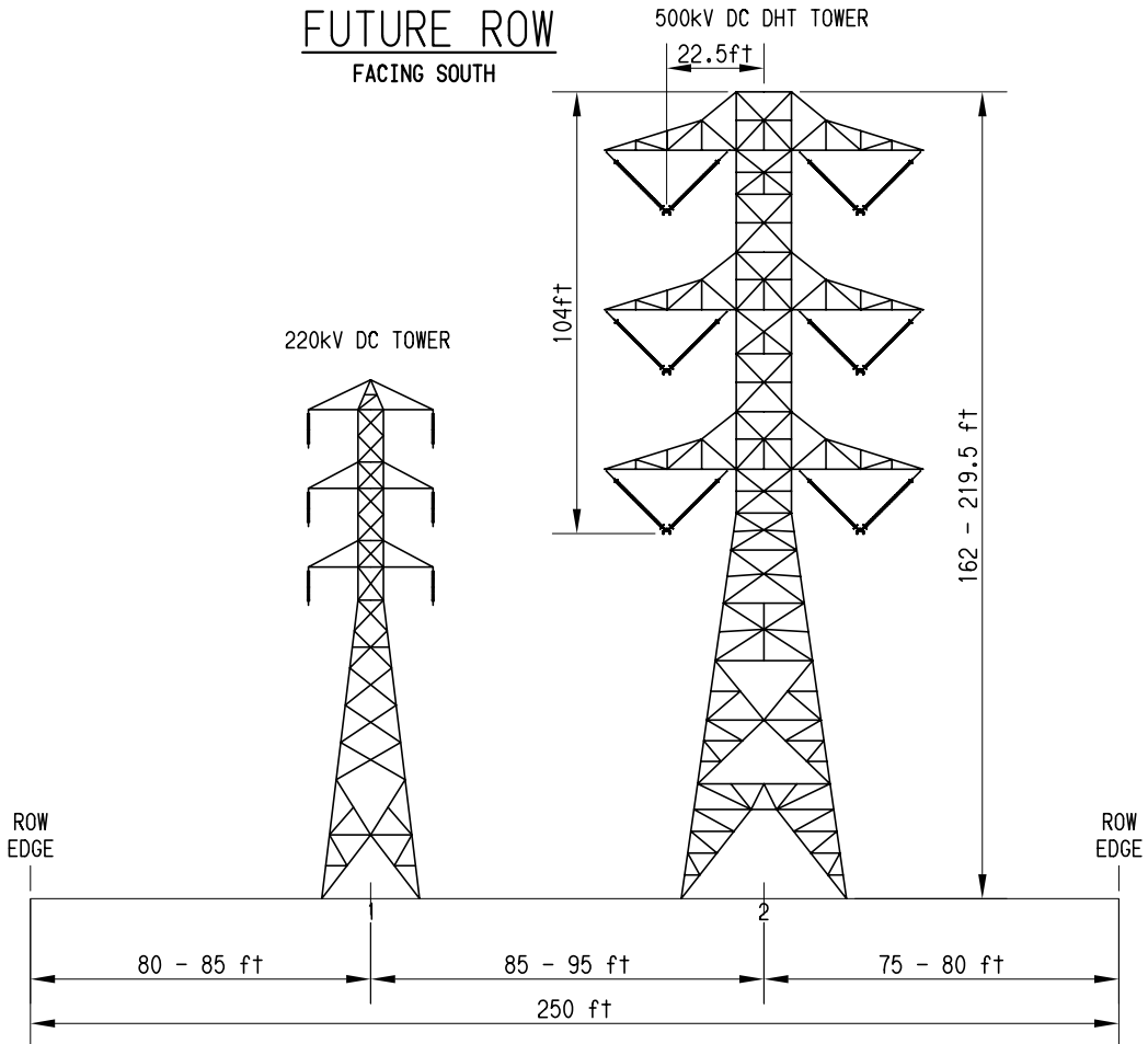
Figure 2.2-22 Segment 7 ROW Cross-Section (S7 MP 4.3 to S7 MP 5.1)
