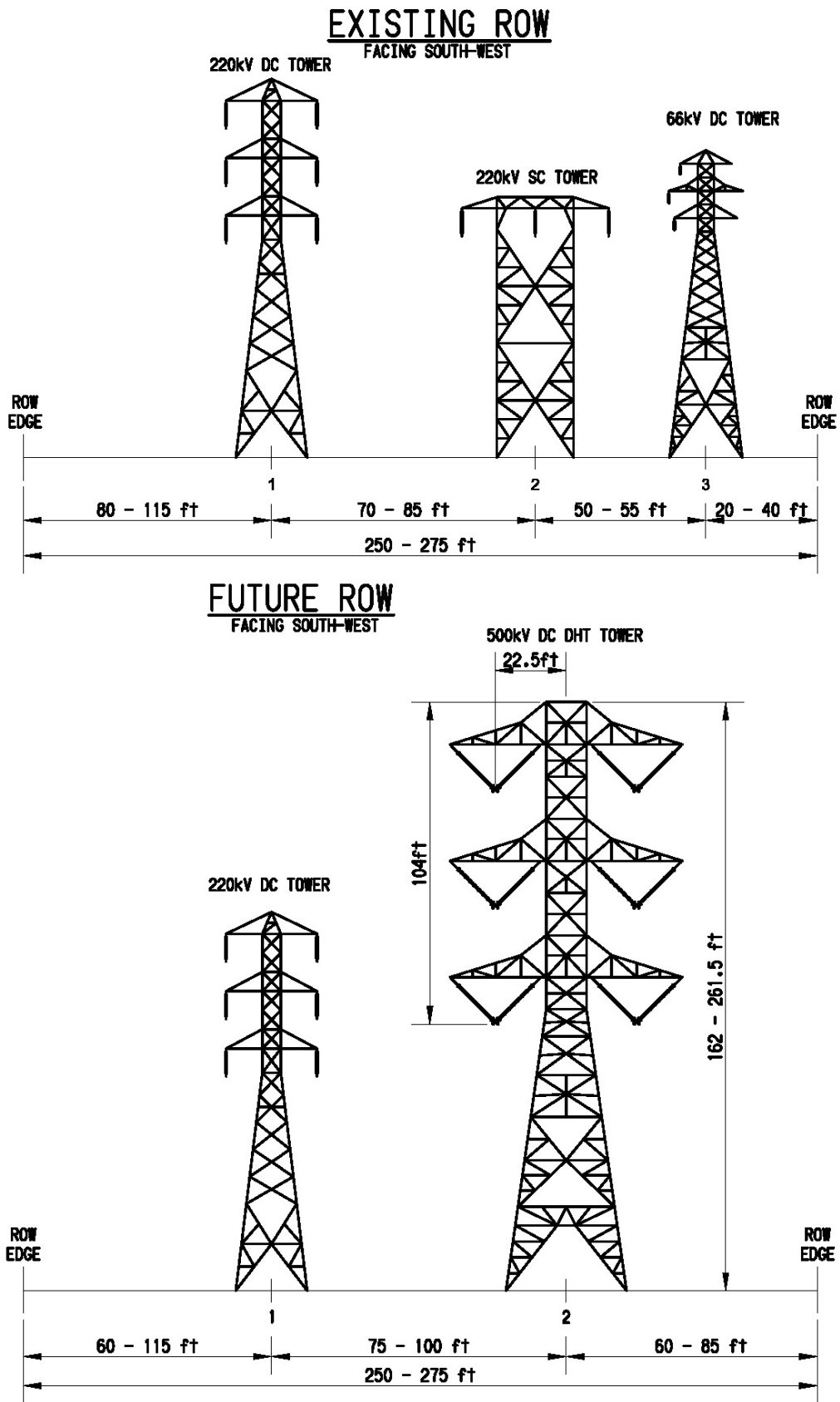
Figure 2.2-23a Segment 7 ROW Cross-Section (S7 MP 5.1 to S7 MP 8.3)
