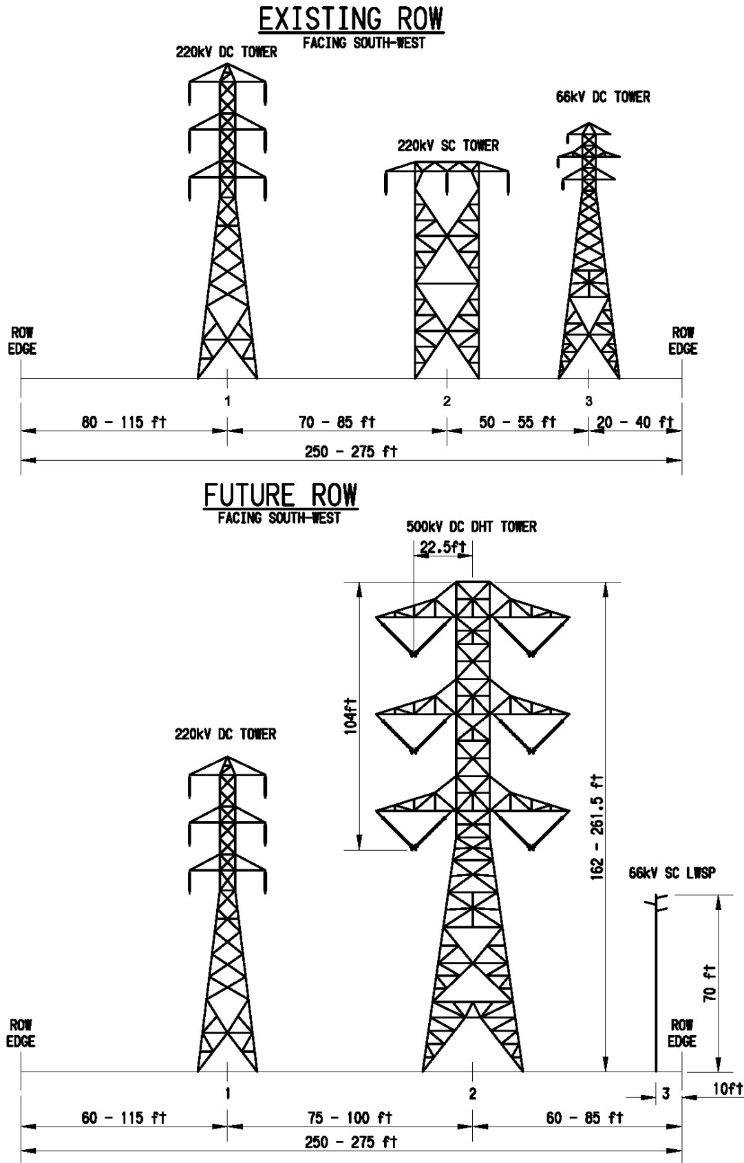
Figure 2.2-23b Segment 7 ROW Cross-Section (S7 MP 8.3 to S7 MP 10.1)
